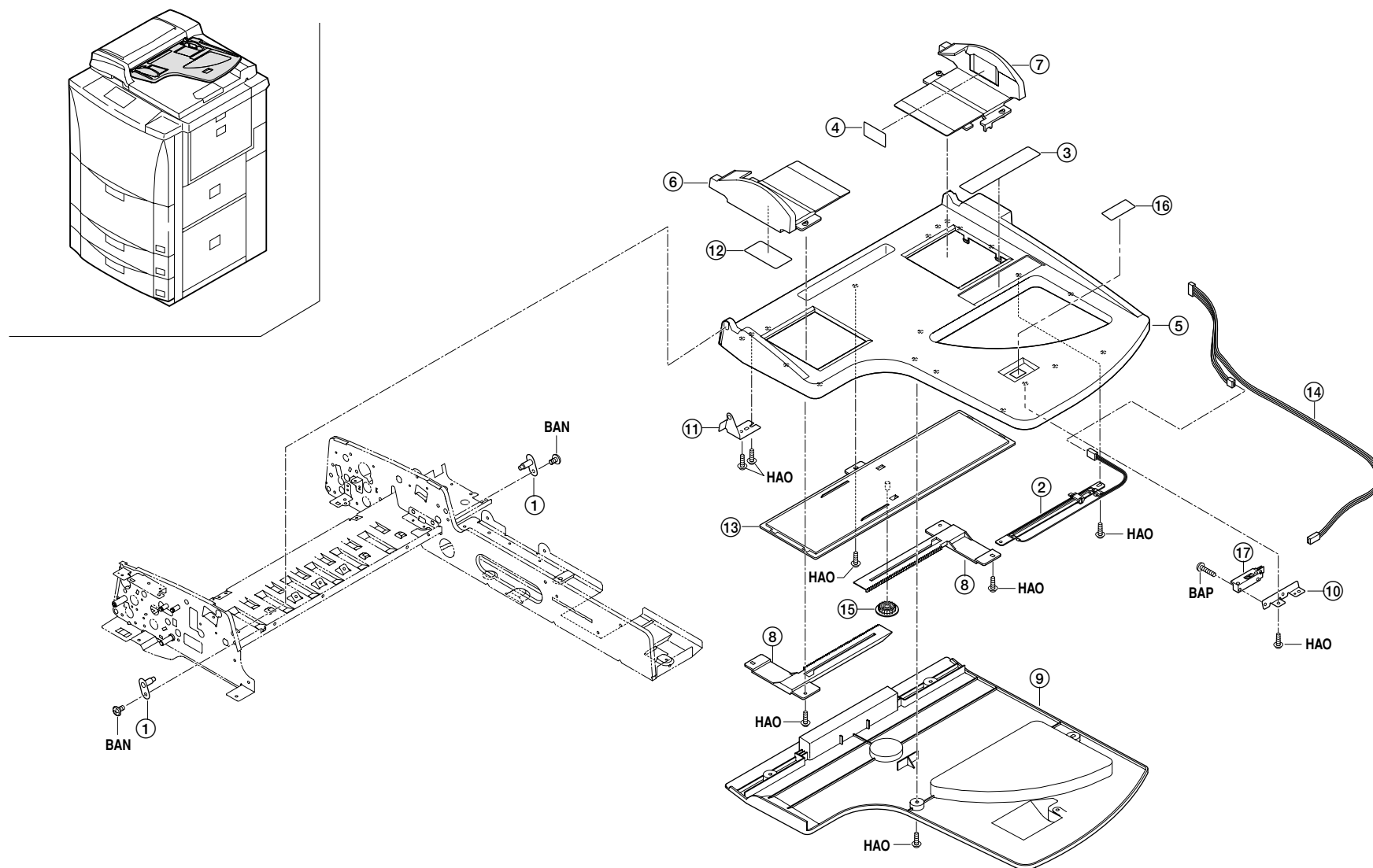
FIG.38 PAPER FEED-IN SECTION
