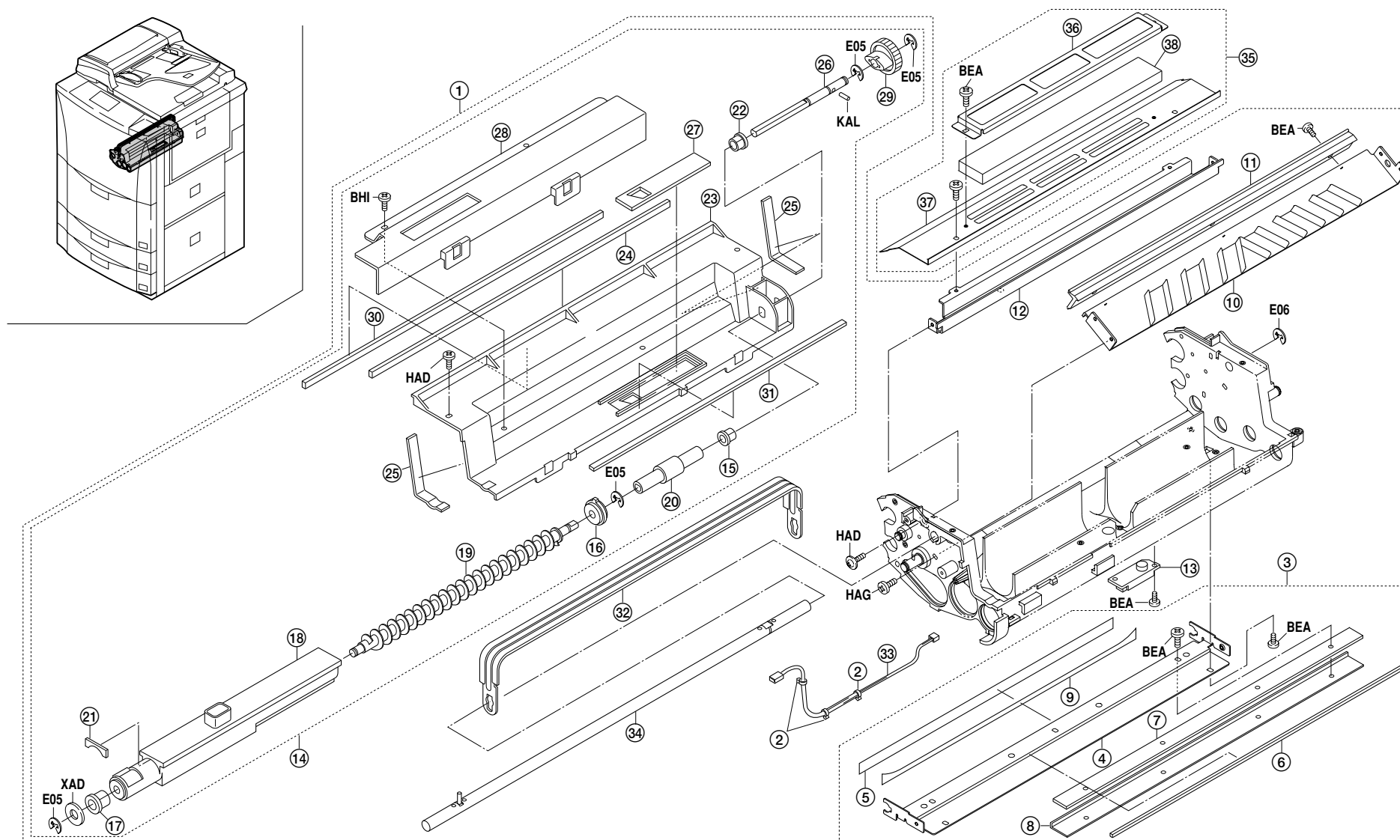
FIG.17 DEVELOPING SECTION I
