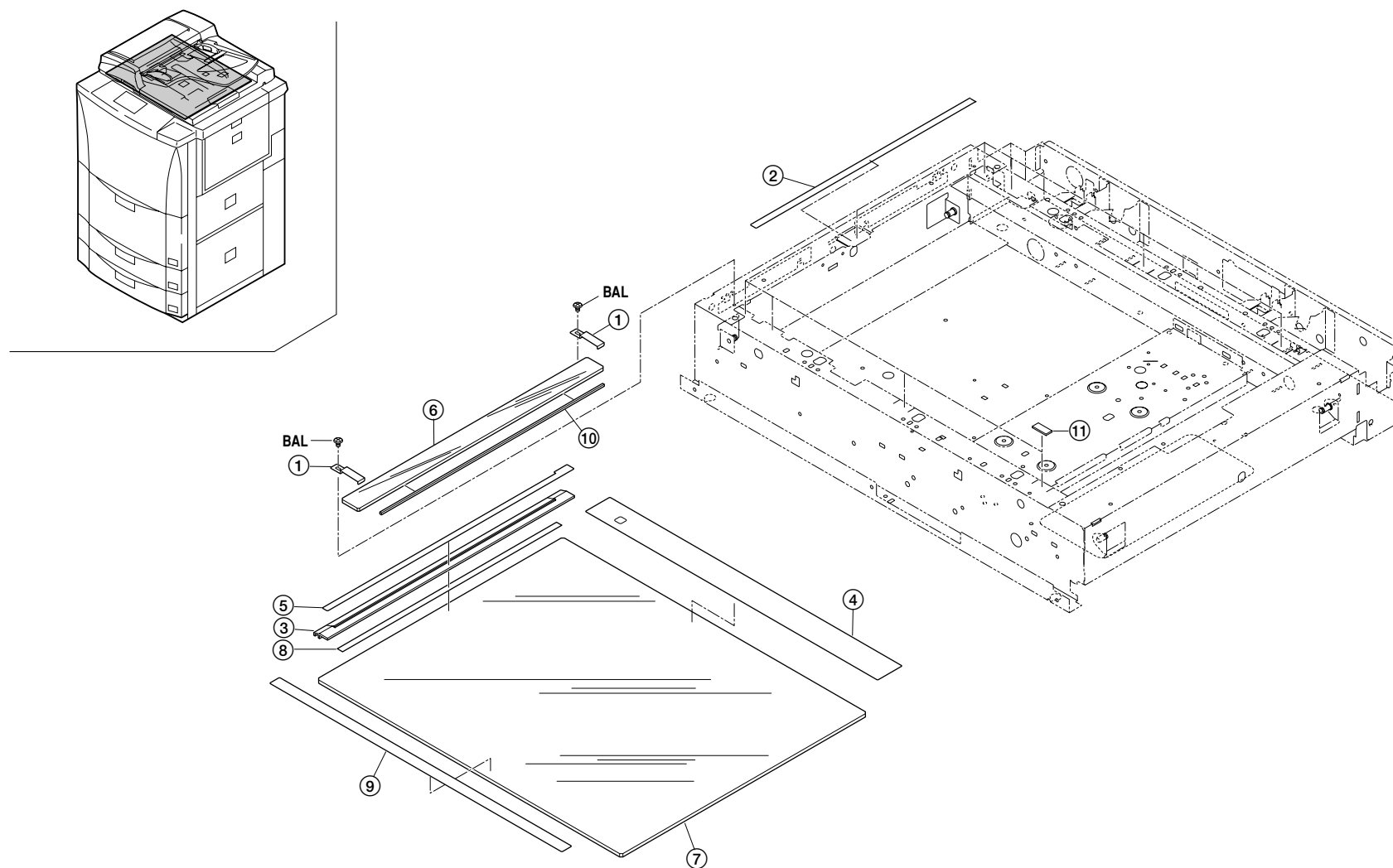
FIG.13 ORIGINAL SET SECTION
