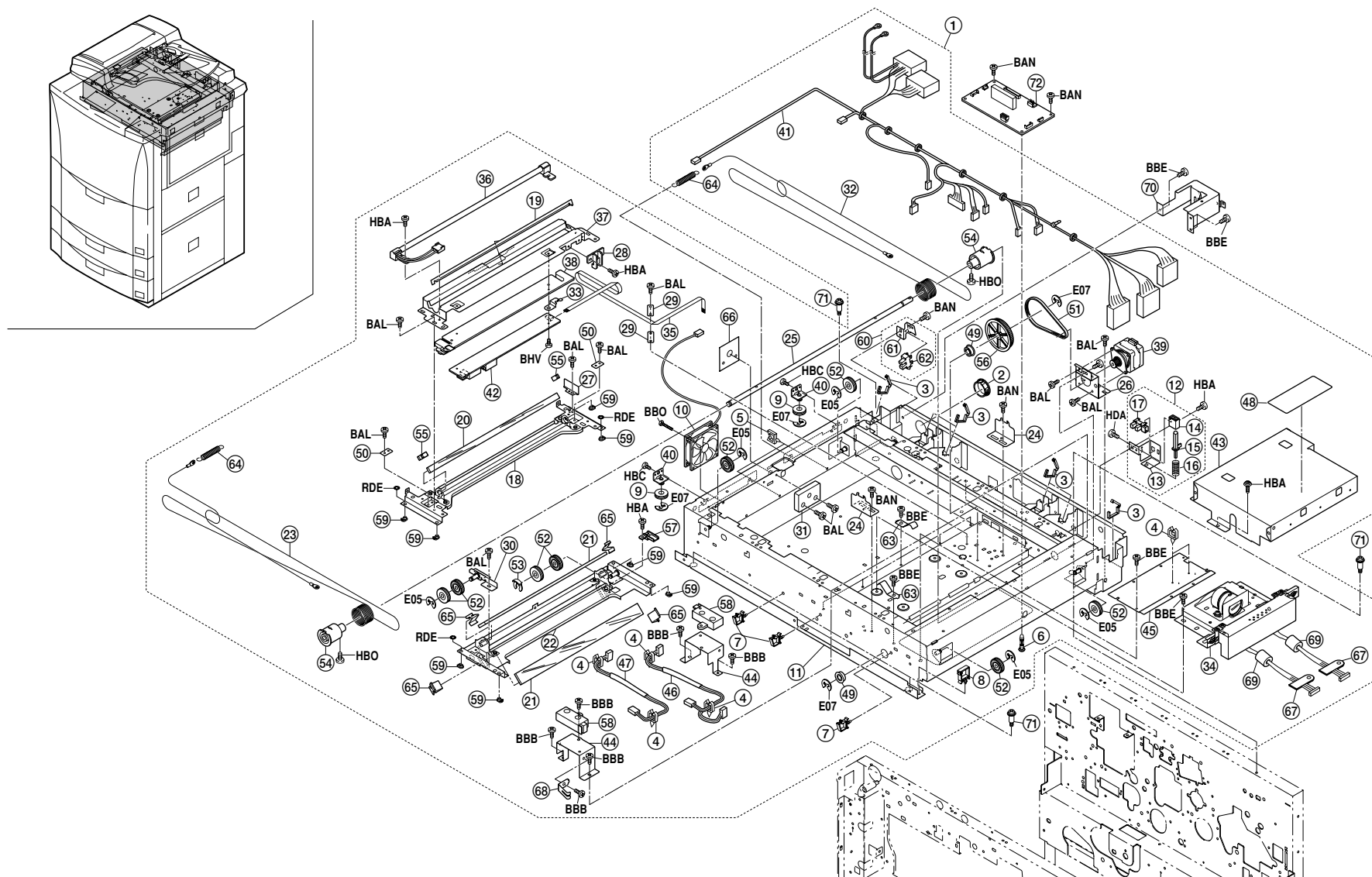
FIG.14 OPTICAL SECTION
