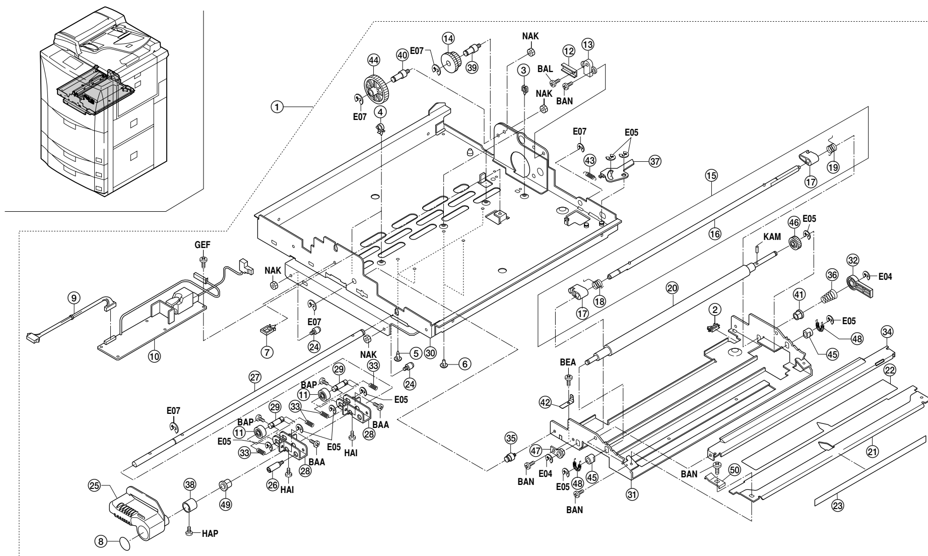
FIG.12 PAPER CONVEYING SECTION II
