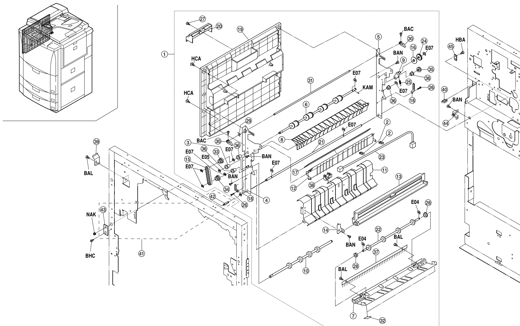
FIG.31 PAPER EJECT SECTION
