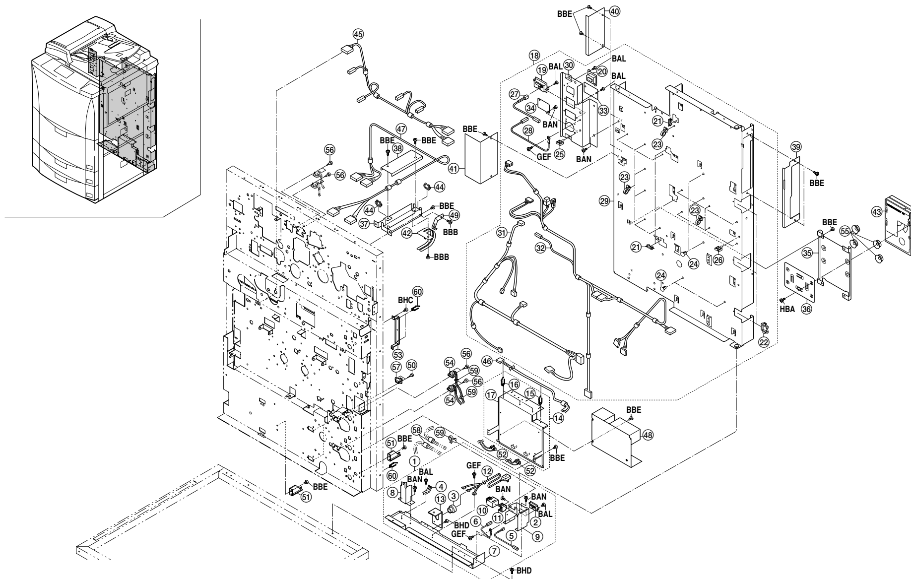
FIG.32 ELECTRICAL COMPONENTS I (120V)
