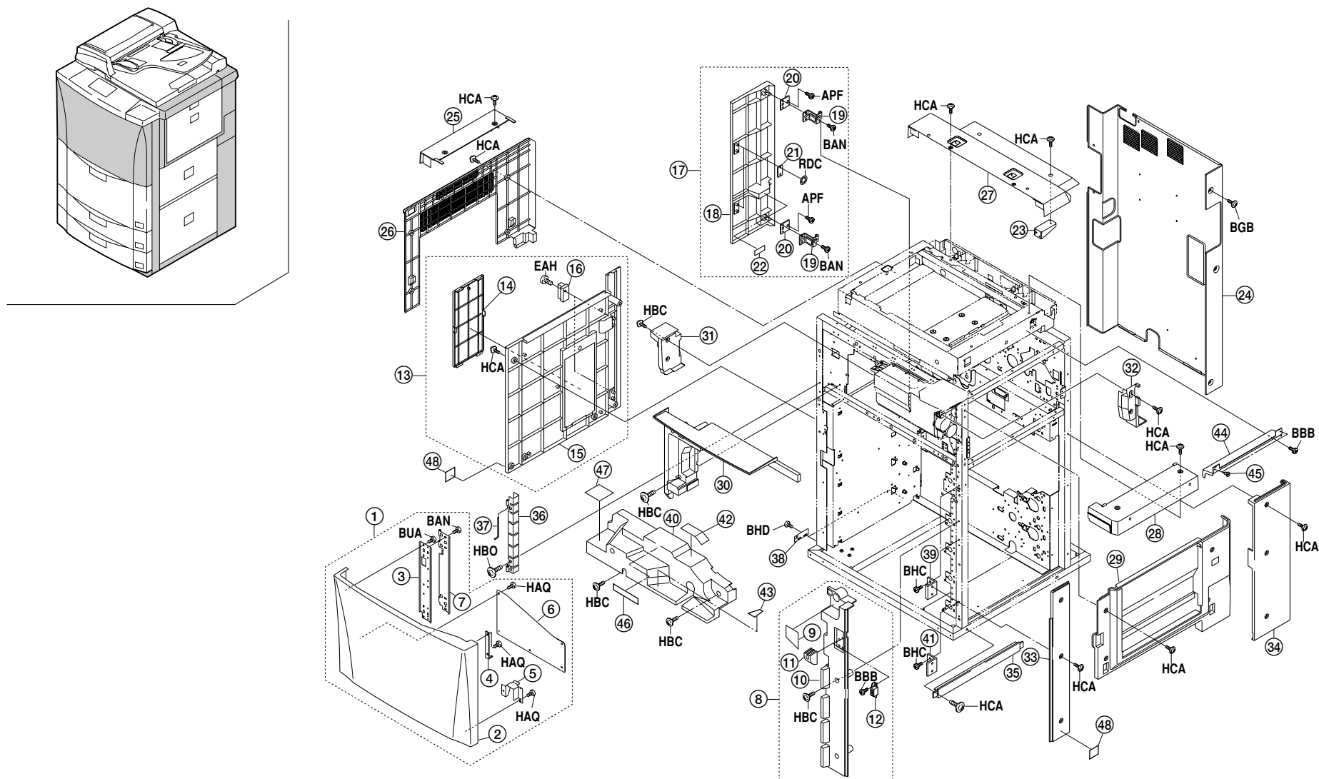
FIG. 1 EXTERIOR COVERS
