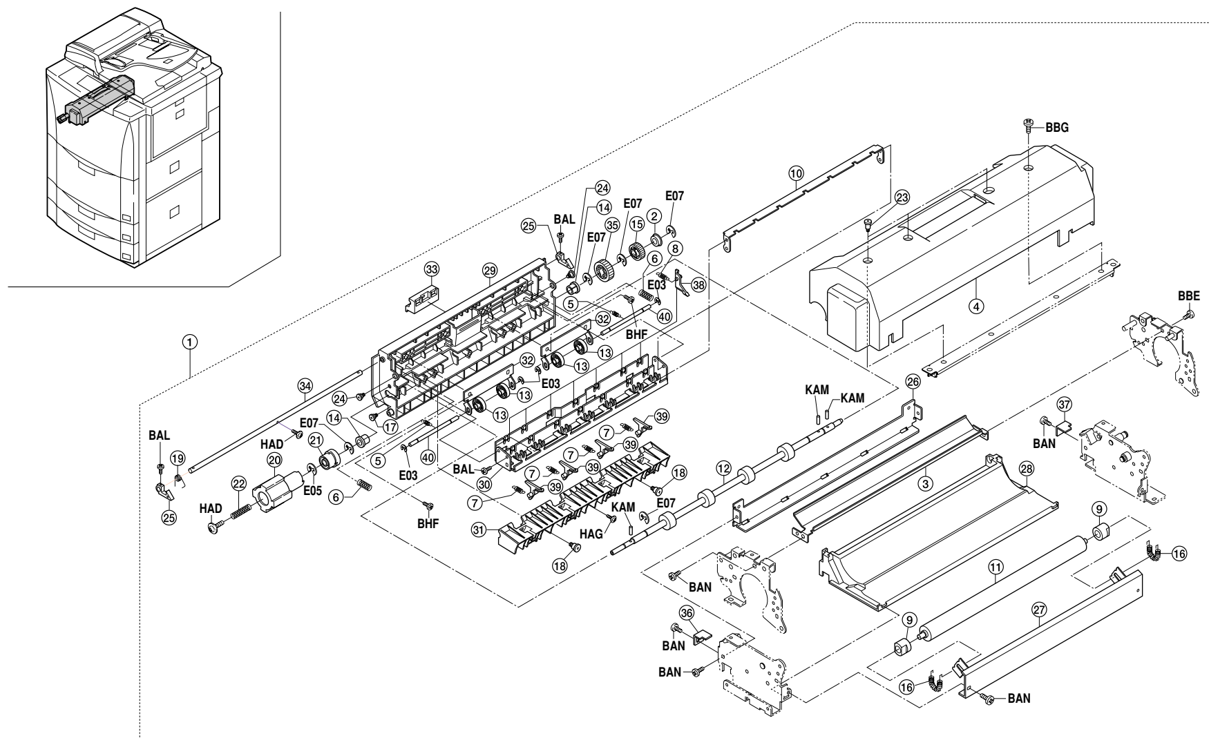
FIG.22 FIXING SECTION I
