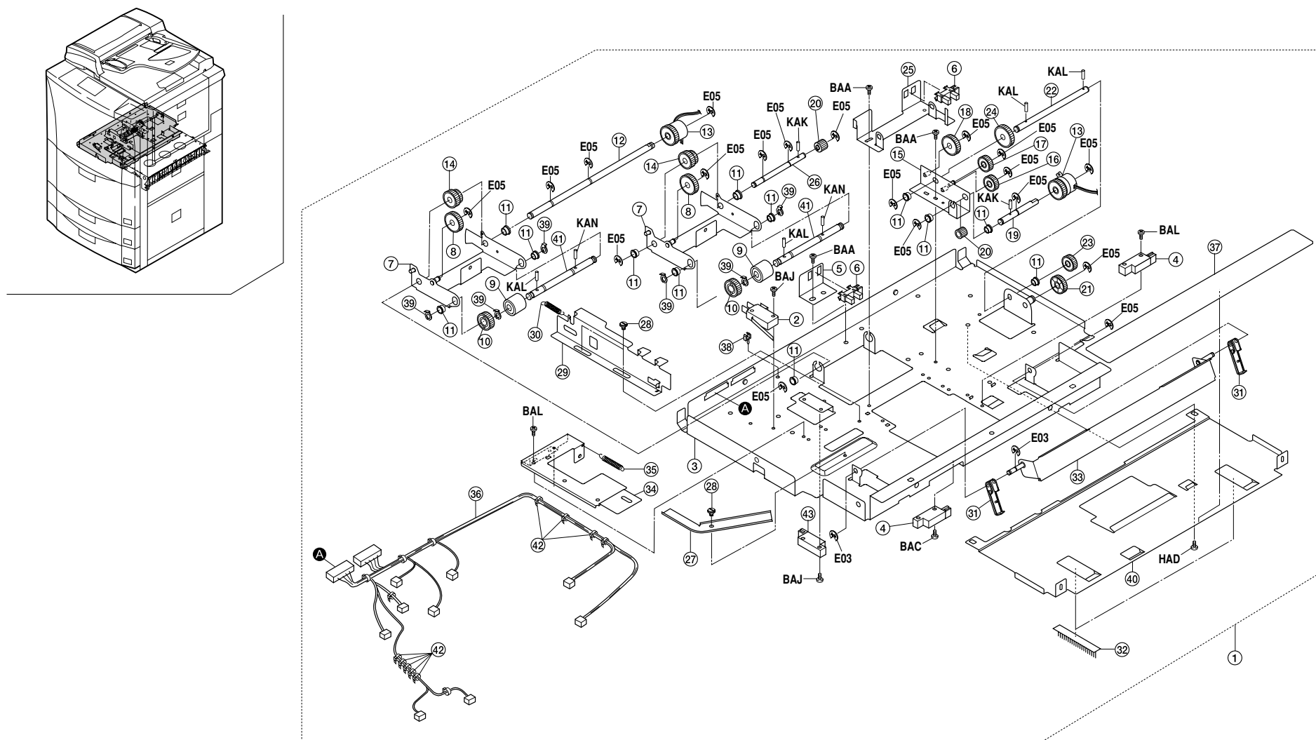
FIG. 6 DECK UNIT III
