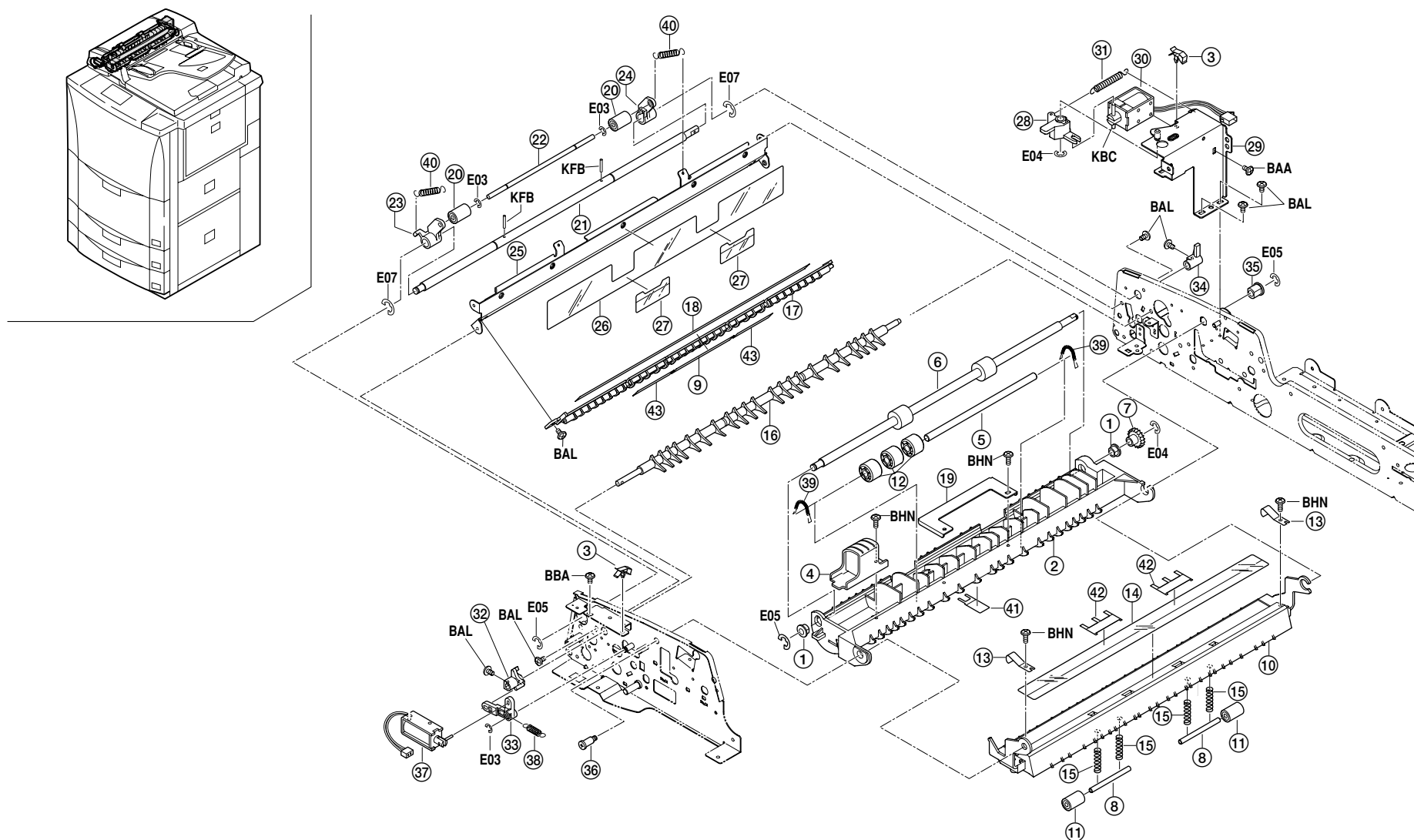
FIG.40 REVERSING SECTION
