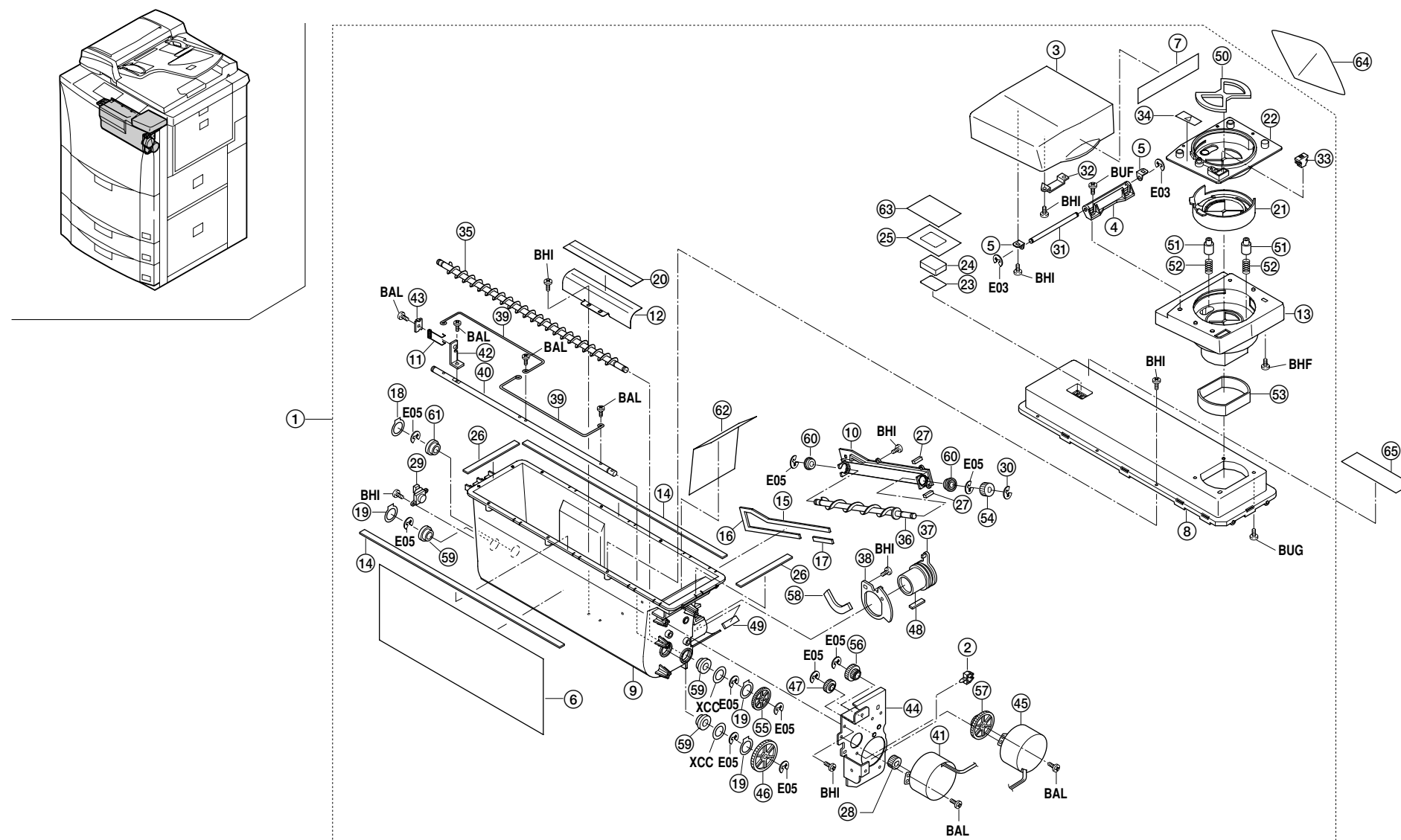
FIG.19 TONER HOPPER SECTION
