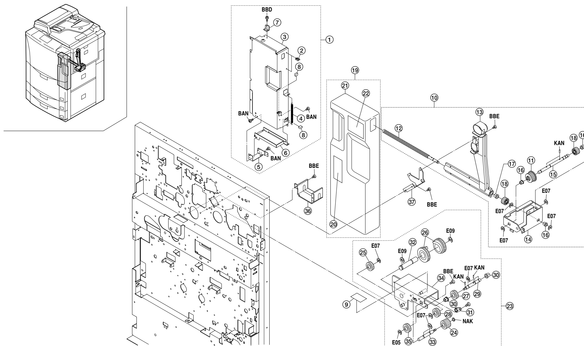
FIG.21 CLEANING SECTION II
