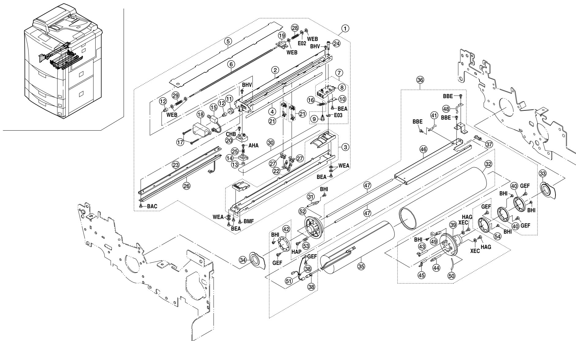
FIG.15 IMAGE FORMATION SECTION I
