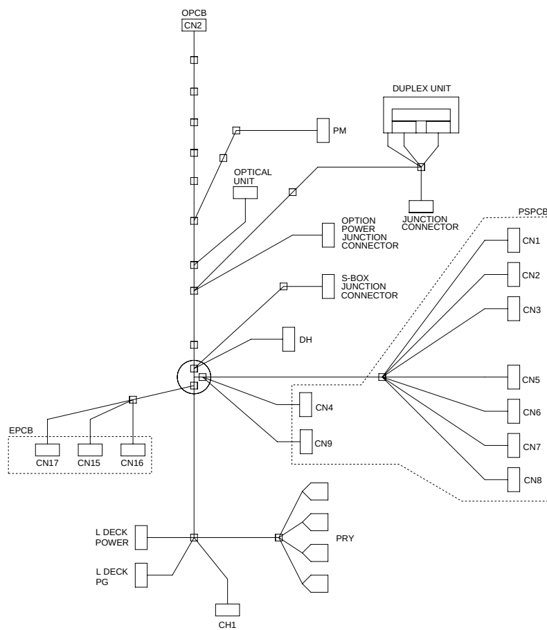
① 2A027350 WIRE,SECONDARY
