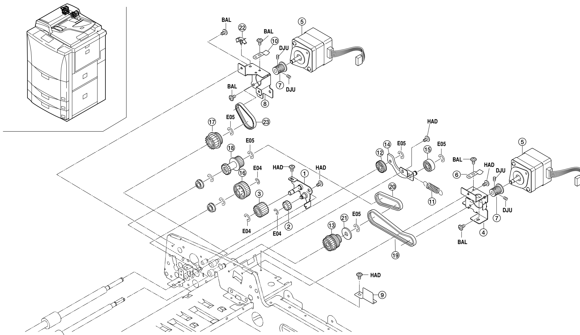
FIG.42 DRIVING SECTION
