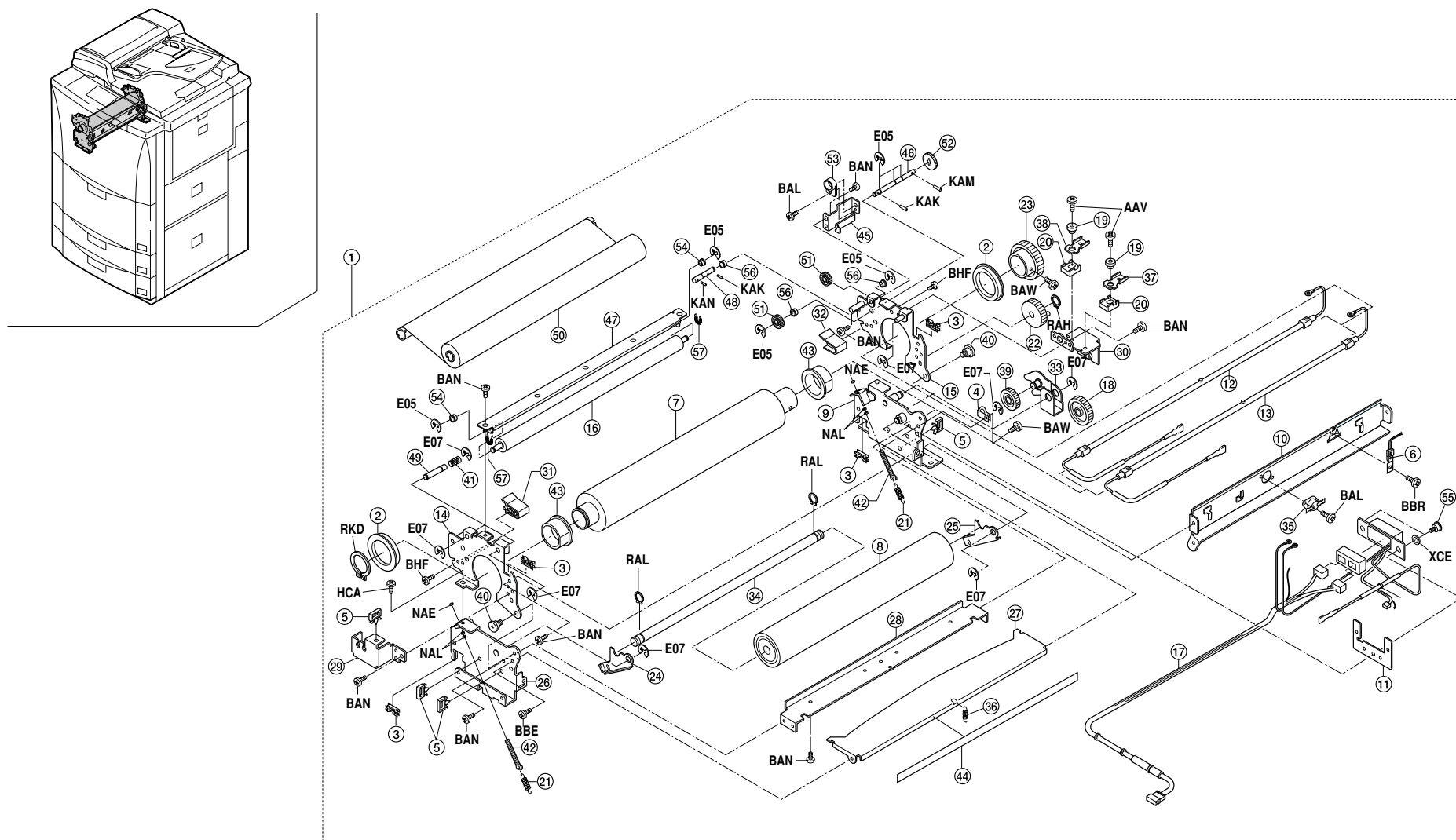
FIG.23 FIXING SECTION II
