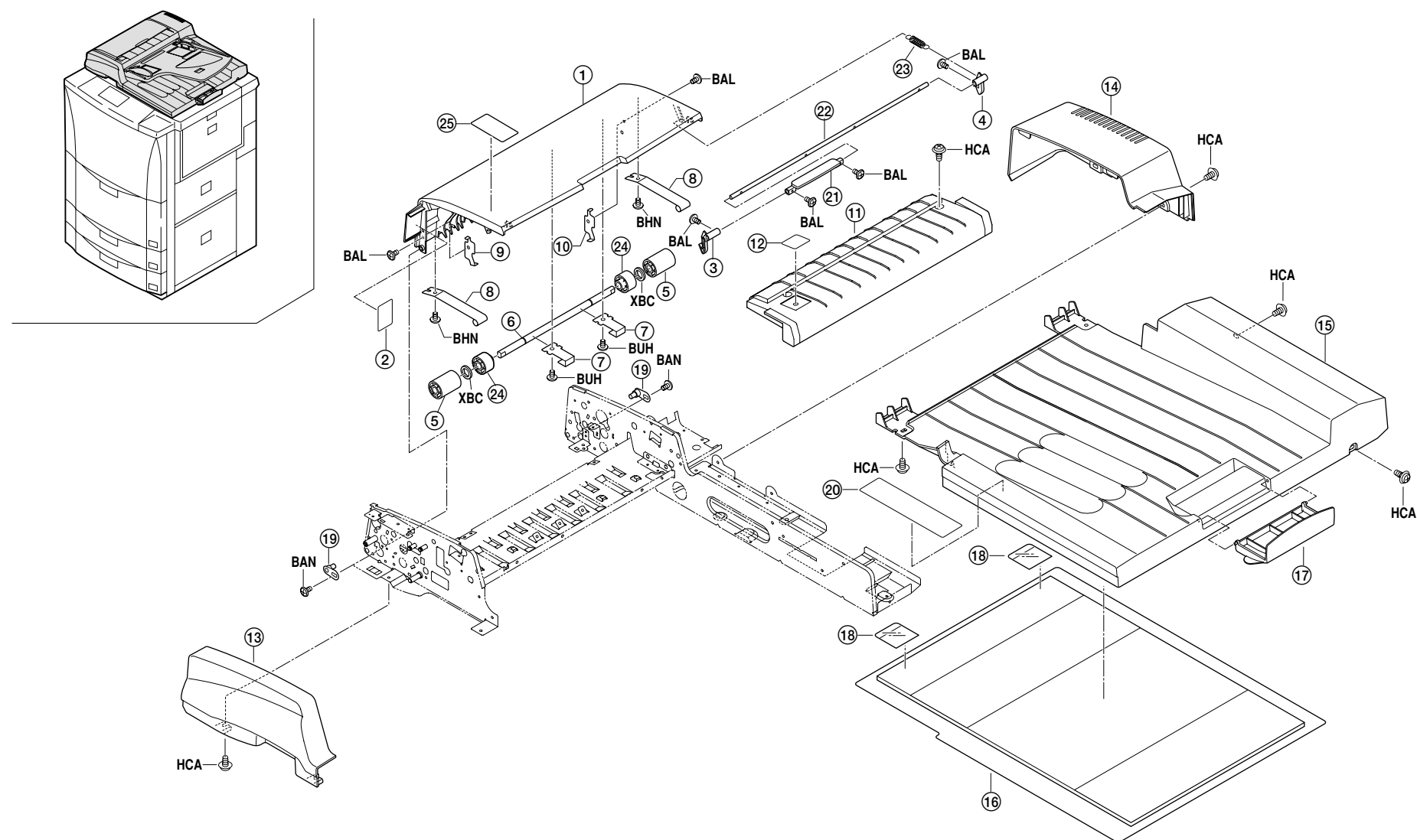
FIG.36 EXTERIOR COVERS
