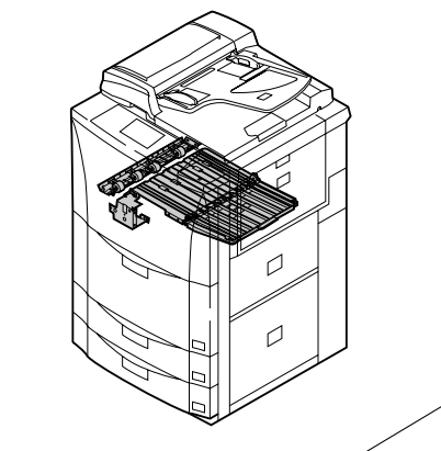
FIG.28 DUPLEX UNIT II
