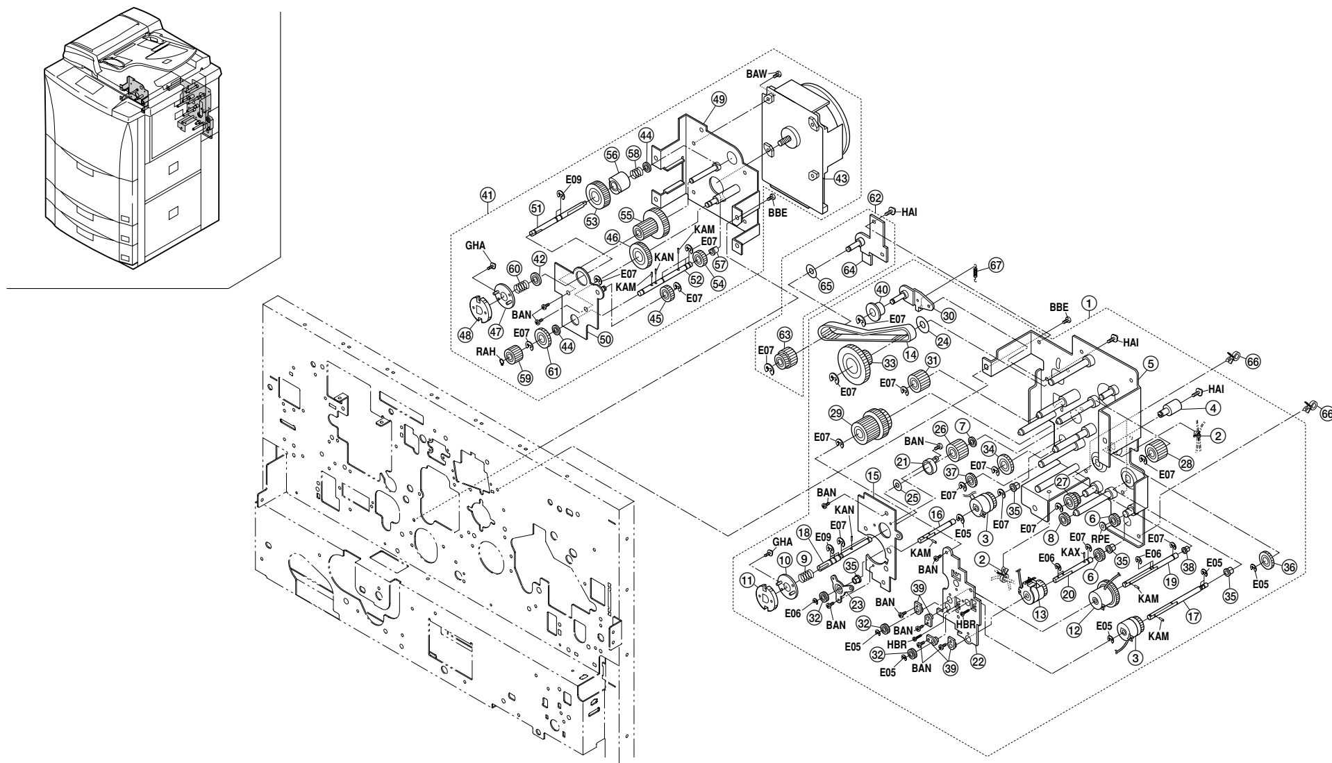
FIG.24 DRIVING, COOLING SECTION I
