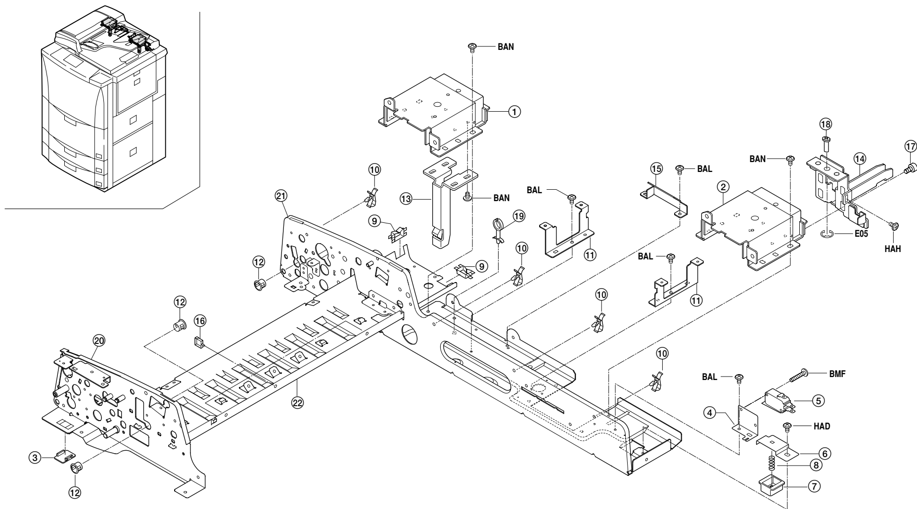
FIG.37 FRAMES
