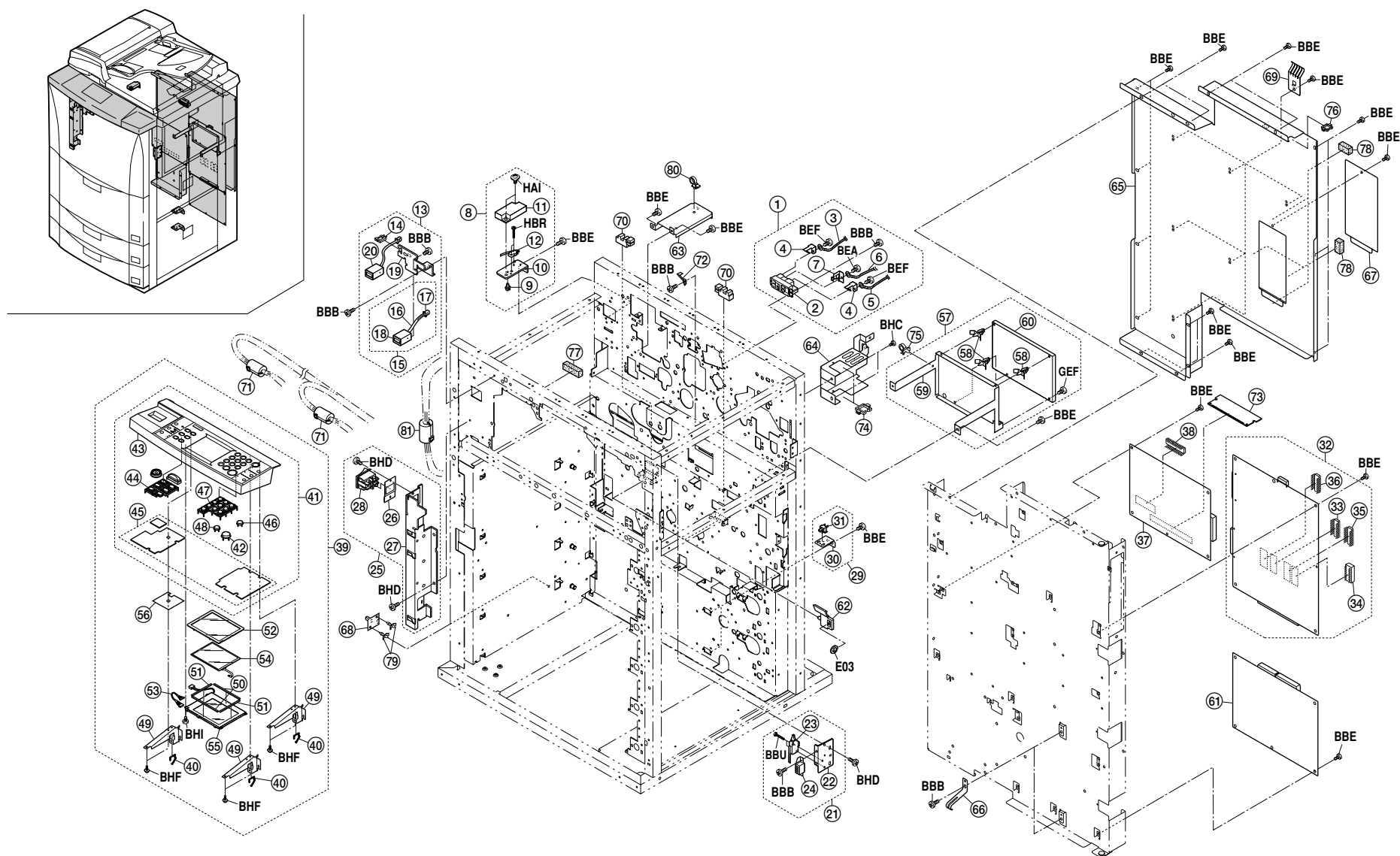
FIG.33 ELECTRICAL COMPONENTS II
