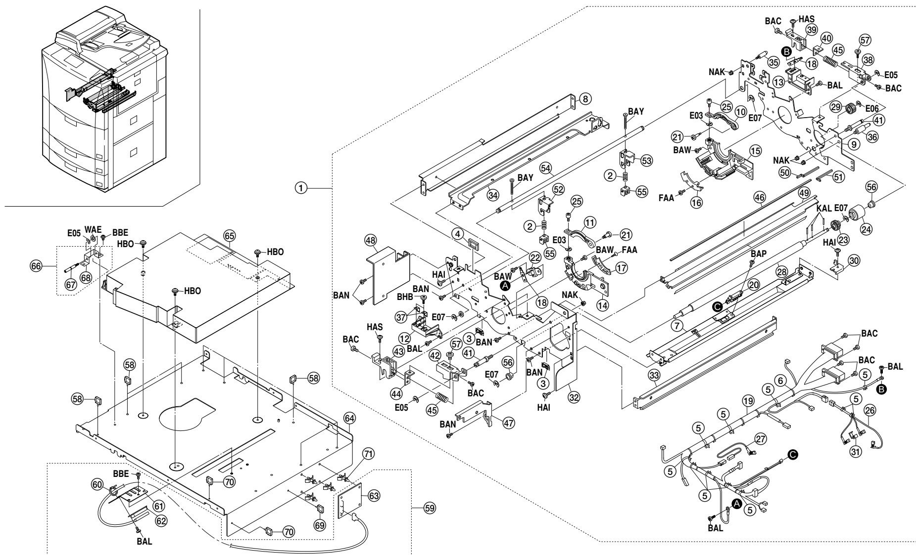
FIG.16 IMAGE FORMATION SECTION II
