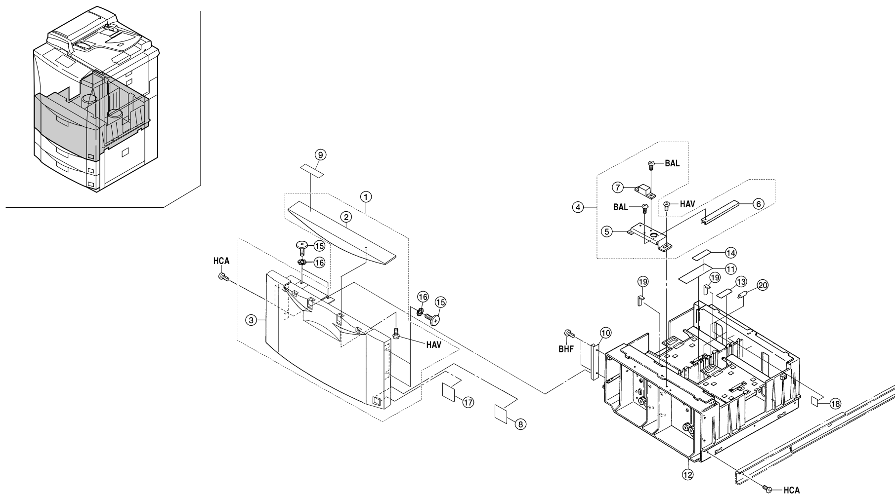
FIG. 4 DECK UNIT I
